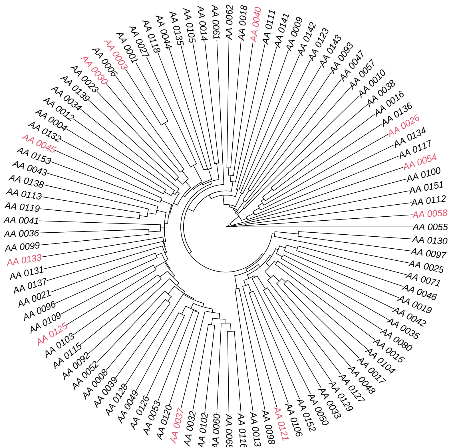
UPGMA Tree (Bray–Curtis) by Insulin
